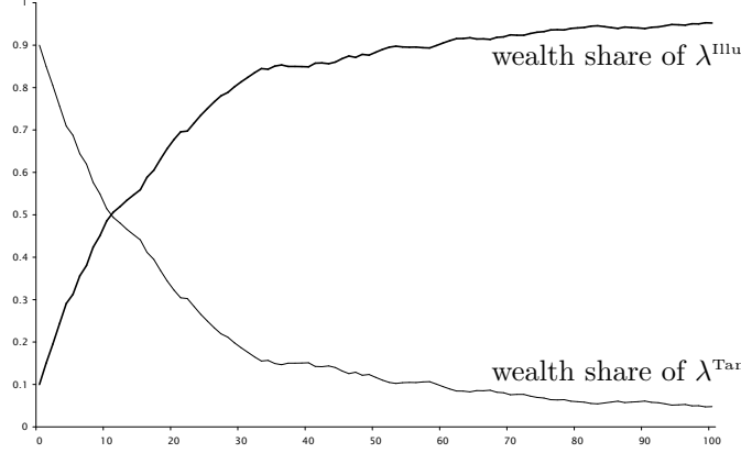
Figure 5: Dynamics of wealth shares in a market with an illusionary diversification strategy \lambda^{\text{Illu}} and the tangency mean-variance rule \lambda^{\text{Tan}} .
