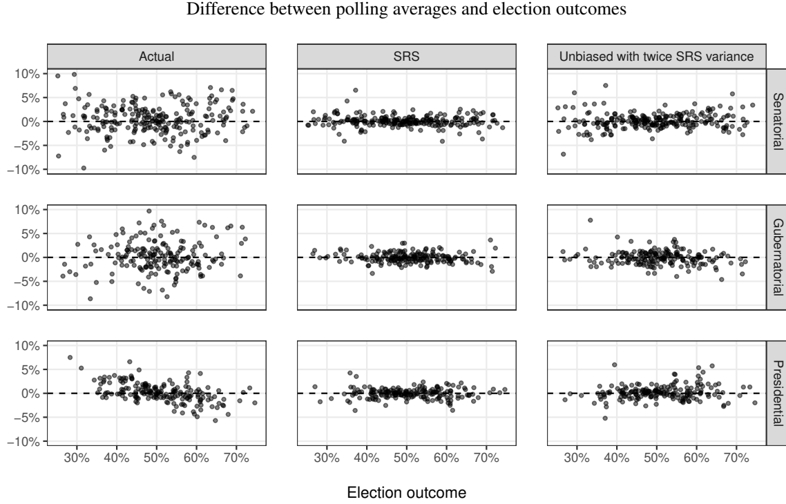
Figure 3: Difference between polling averages and election outcomes (i.e., Republican share of the two-party vote), where each point is an election. The left panel shows results for the real polling data; the middle panel shows results for a synthetic dataset of SRS polls; and the right panel shows results for a synthetic dataset of polls that are unbiased but that have twice the variance of SRS.
