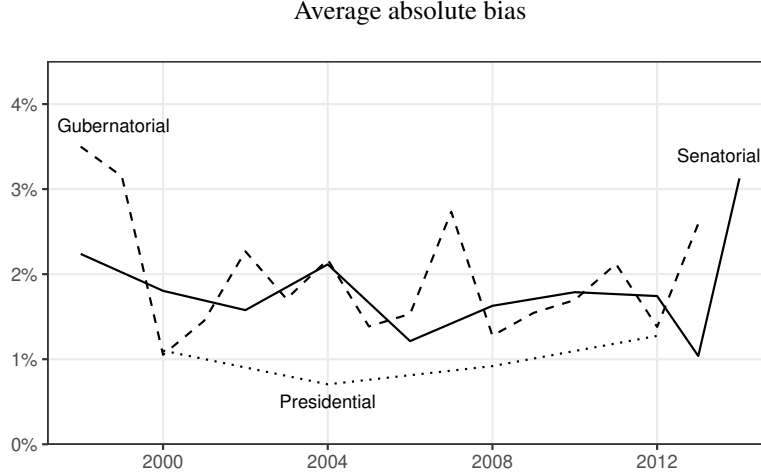
Figure 5: Model-based estimates of average absolute bias show no consistent time trends across election cycles.
