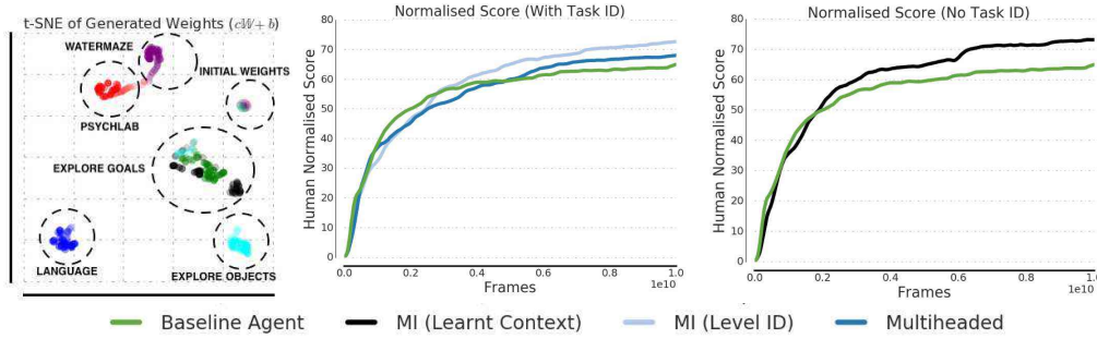
Figure 4: (a) A t-SNE plot of the generated weights from an \mathcal{M} layer. (b) Human normalised performance (capped at 100) when using task ID as context to an \mathcal{M} layer. (c) Using a learnt context instead.
