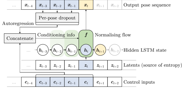
Fig. 3. Schematic of autoregressive motion generation with MoGlow. Inputs are blue, outputs yellow. Dropout is only applied at training time.
