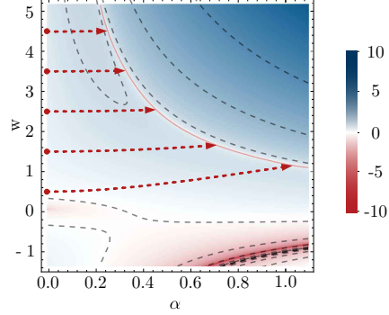
Figure 2: Contour plot of the log gradient norm, \log \|\partial \mathcal{C}\|_2 , over the network weight w and the residual weight \alpha during the training of the linear function x_{L=5} = 50 \times x_0 via gradient descent using a training set of x_0 = \{1, 1.1, \dots, 1.8\} . Gradient descent trajectories initialized at \alpha = 0 are shown in red for five different initial w 's. The trajectory dynamics avoid the poorly conditioned regions around \alpha \approx 1 and converge to the solution \alpha w \approx 1.2 .
