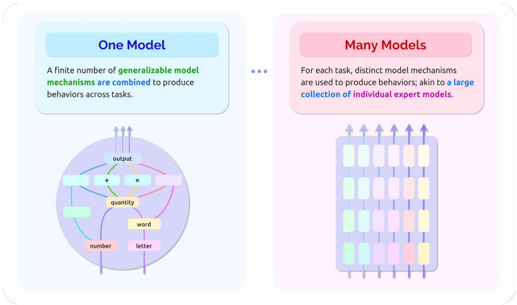
Fig. 23. One model-many model nature of foundation models: A central question for the interpretability of a foundation model is to understand where it is located on the spectrum between one model and many models . As one model, behavior can be made interpretable by identifying and characterising the finite number of generalizable model mechanisms that the model uses to produce behaviors across tasks (e.g., mechanisms that assign meaning to words, compare quantities, and perform arithmetic). As many models, explanations of model behavior in one task are not necessarily informative about behavior in other tasks; thus requiring to study behavior independently in each task.
