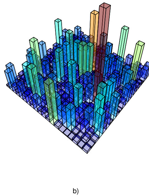
Figure 4 The Lorenz curve (a) and 400 samples (b) from a beta distribution resulting from a familial relative risk of 2.3 and E[P] = 0.01 , representing Parkinson's disease.
