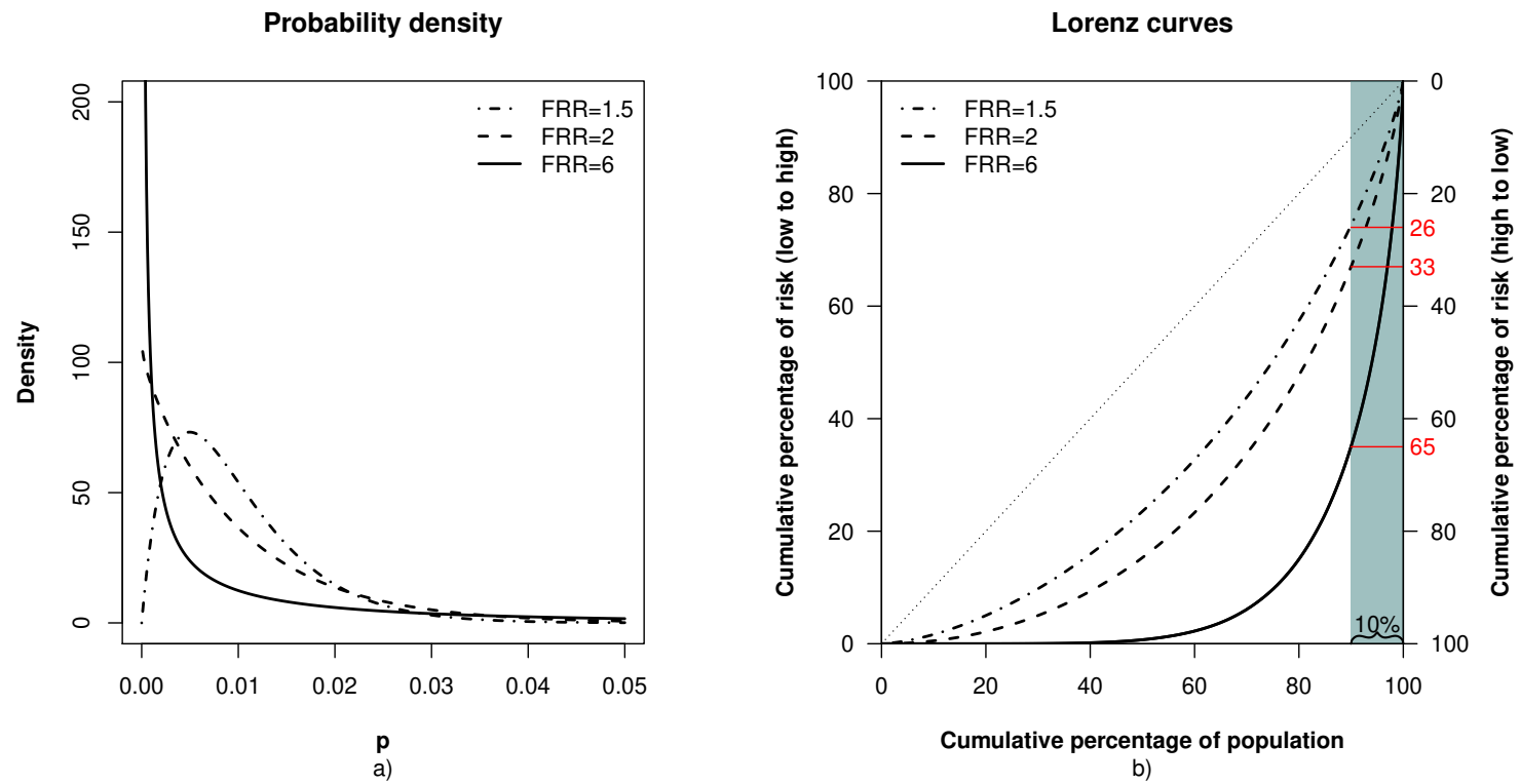
Figure 5 The distribution (a) of a beta distributed variable P , and its corresponding Lorenz curve (b), for three selected familial relative risks (FRRs). The expected value of P is set to 0.01. The 10% at highest risk (shaded area) account for 26%, 33%, and 65% of the diagnoses in the three scenarios, respectively.
