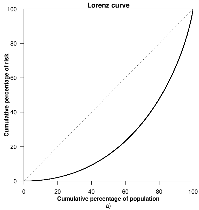
Figure 4 The Lorenz curve (a) and 400 samples (b) from a beta distribution resulting from a familial relative risk of 2.3 and E[P] = 0.01 , representing Parkinson's disease.
