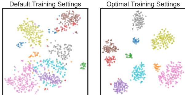
Figure 4. The default Inception training settings produce a suboptimal feature space. Low dimensional embeddings of Oxford 102 Flowers using t-SNE [53] on features from the penultimate layer of Inception v4, for 10 classes from the test set. Best viewed in color.
