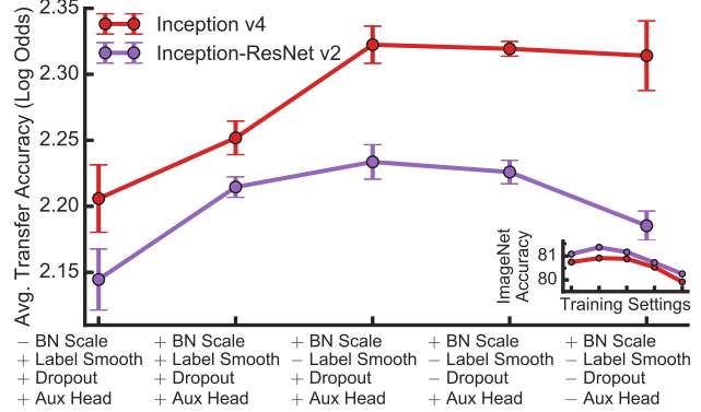
Figure 5. ImageNet training settings have only a minor impact on fine-tuning performance. Each point represents transfer accuracy for a model pretrained and fine-tuned with the same training configuration, labeled at the bottom. Axes follow Figure 3. See Appendix C.2 for performance of models pretrained with regularization but fine-tuned without regularization.
