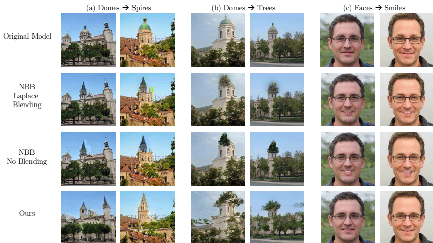
Fig. 4: Adding and replacing objects in three different settings. (a) Replacing domes with an angular peaked spire causes peaked spires to be used throughout the model. (b) Replacing domes with trees can generate images unlike any seen in a training set. (c) Replacing closed lips with an open-mouth smile produces realistic open-mouth smiles. For each case, we show the images generated by an unchanged model, then the edit propagation results, with and without blending. Our method is shown in the last row.
