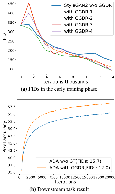
Figure 7. (a) FID score graph of multiple experiments with GGDR in the early training phase on LSUN Cat. (b) Validation pixel accuracy on the ADE20K segmentation task with the frozen discriminator trained with and without GGDR.
