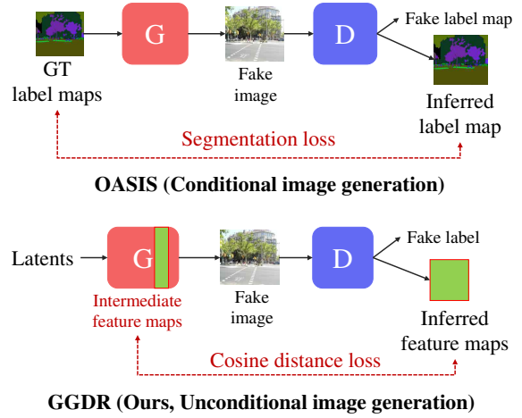
Figure 1. Comparison of how to provide semantic information between OASIS and our method. OASIS enhance the discriminator with the ground truth label maps in conditional image generation setting. GGDR, on the other hand, aims at unconditional image synthesis, and uses the generator feature maps instead of human-annotating label maps.
