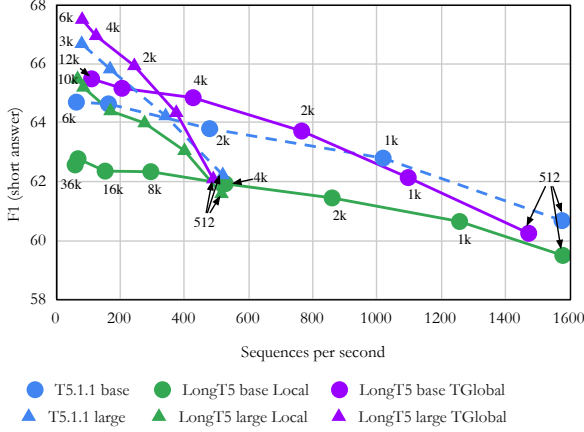
Figure 4: Speed versus Performance on NQ (short-answer F1), for T5, LongT5 with Local Attention and LongT5 with TGlobal attention, for different input sequence lengths. Input lengths start at 512, and go as far as possible before running out of memory. Measurements taken with batch size 128, on 4x8 TPUv3 slices.
