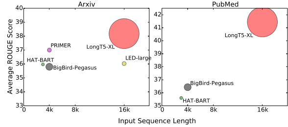
Figure 1: The average ROUGE score ( (R-1 + R-2 + R-L)/3 ) of LongT5 and baseline models on arXiv and PubMed summarization tasks (Cohan et al., 2018) with different input length ( x axis). Baseline models: HAT-BART (Rohde et al., 2021), BigBird-PEGASUS (Zaheer et al., 2020b), PRIMER (Xiao et al., 2021), LED (Beltagy et al., 2020). The size of circle roughly indicates the # of parameters for each model.
