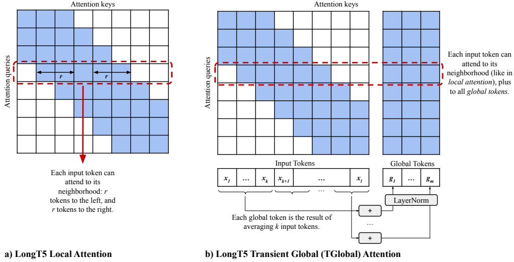
Figure 2: Illustration of the two attention mechanisms we experimented with in LongT5.
