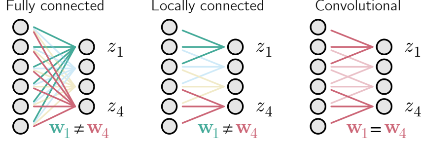
Figure 1: Comparison between layer architectures: fully connected (left), locally connected (middle) and convolutional (right). Locally connected layers have different weights for each neuron z_1 to z_4 (indicated by different colors), but have the same connectivity as convolutional layers.
