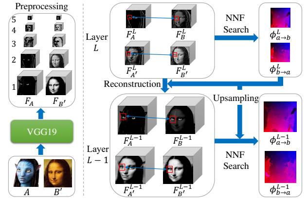
Figure 4: System pipeline.
