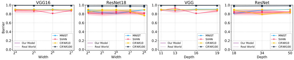
Figure 14: Effect of width and depth on barrier similarity between real world and our model before permutation: VGG and ResNet families. The left two panels shows the effect of width, while the right two panels illustrate the depth. As discussed in section 2, the barrier for VGGs and ResNets, for both real world and our model, is saturated at a high value and does not change.
