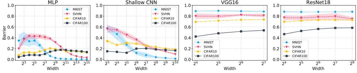
Figure 16: Effect of width on barrier size (Test) . From left to right: one-layer MLP, two-layer Shallow-CNN, VGG-16, and ResNet-18 architectures and MNIST, CIFAR-10, SVHN, CIFAR-100 datasets. When the task is hard (CIFAR10, CIFAR100) the test barrier shrinks. For simpler tasks and large width sizes also the barrier becomes small.
