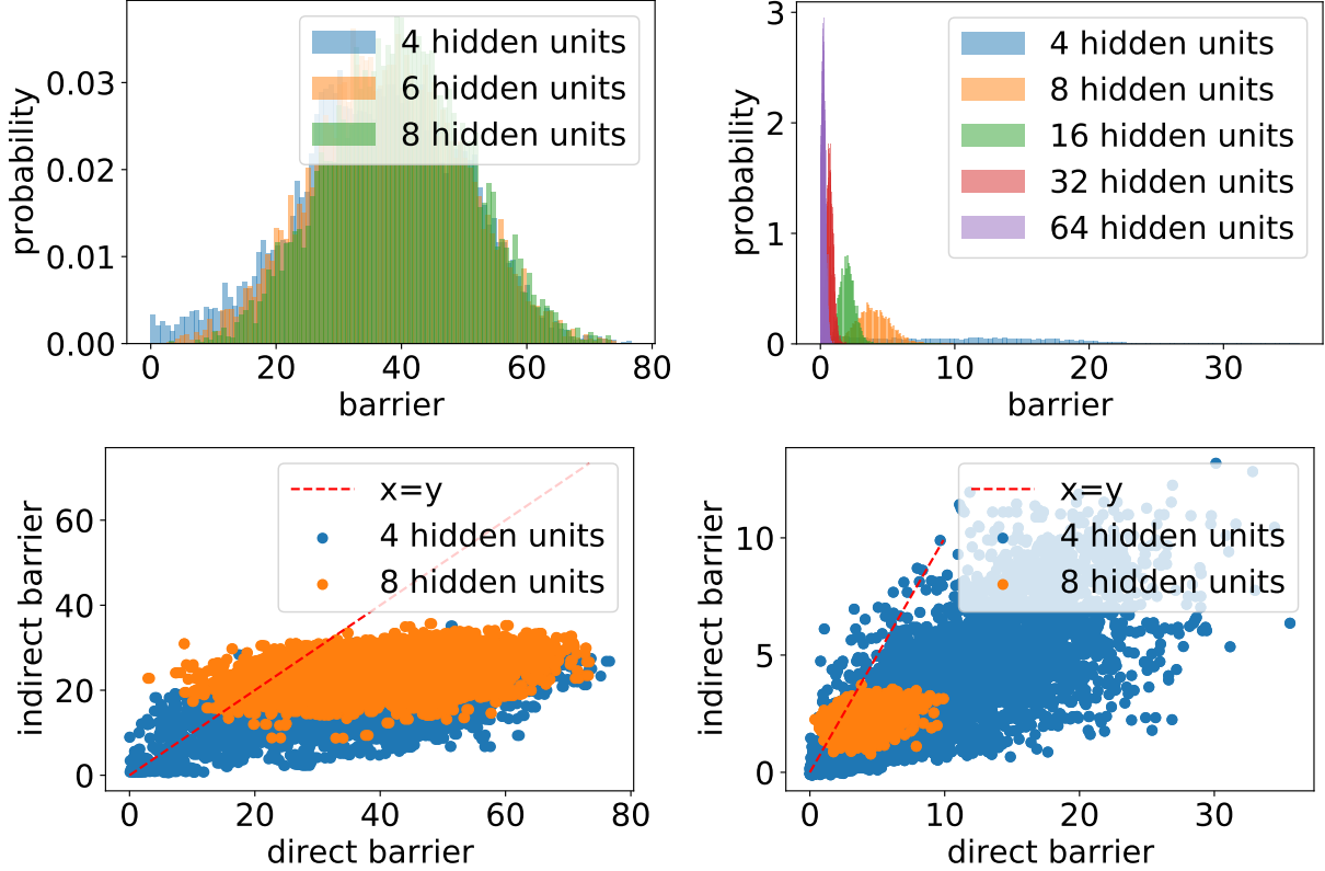
Figure 15: Histogram of barrier values between pairs of 100 networks with the same architecture trained on MNIST starting from different initializations. We find a permutation for each pair that minimizes the barrier. This is done for two layer MLPs and repeated for networks of different sizes. Bottom row: Indirect barrier between two networks A,C is minimum over all possible intermediate points B of maximum of barrier between A, B and barrier between B, C. Left: before the permutation; Right: after the permutation.
