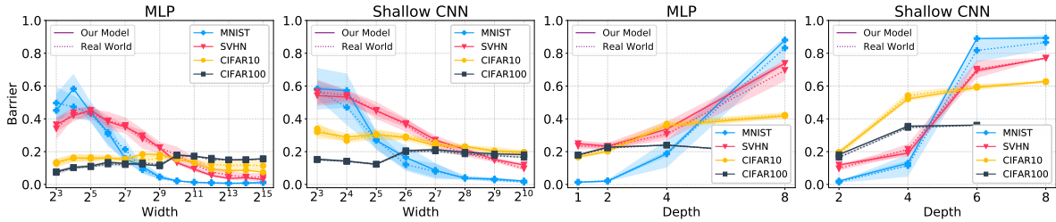
Figure 18: Effect of width and depth on barrier consistency between real world and our model before permutation (Test) . Search space is reduced here i.e. , we take two SGD solutions \theta_1 and \theta_2 , permute \theta_1 and report the barrier between permuted \theta_1 and \theta_2 as found by SA with n = 2 . Similarity of loss barrier between real world and our model is preserved across model type and dataset choices as width and depth of the models are increased.
