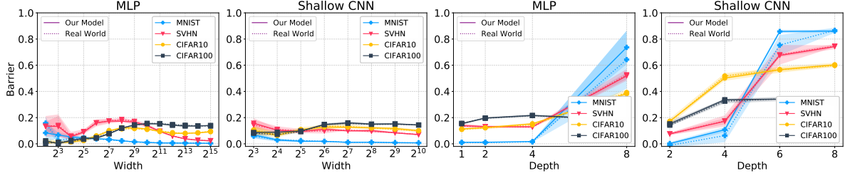
Figure 19: Effect of width and depth on barrier consistency between real world and our model after permutation (Test) . We observe that reducing the search space makes SA more successful in finding the permutation \{\pi\} to remove the barriers. Specifically, SA could indeed find permutations across different networks and datasets that when applied to \theta_1 result in almost zero test barrier e.g. , MLP across MNIST dataset where depth is 1 and width is larger than 2^6 , MLP for MNIST where depth is 2 and 4, and width is 2^{10} , Shallow-CNN for MNIST where depth is 2, Shallow-CNN for SVHN where depth is 2 and width is 2^{10} .
