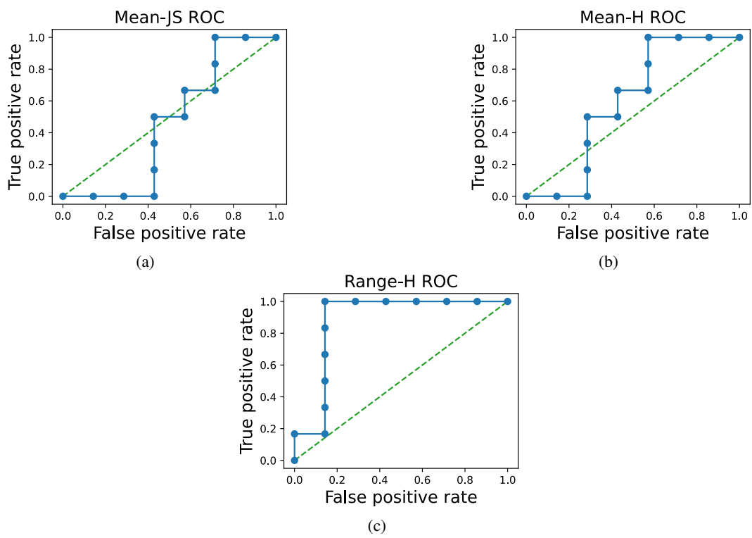
Figure 13: ROC curves for COVID - ontological.
