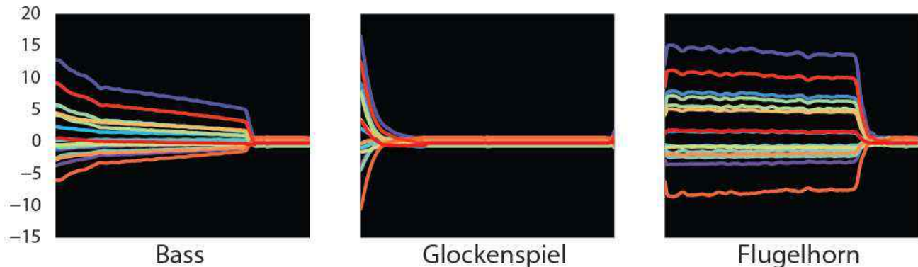
Figure 6. Temporal embeddings for three different instruments. The different colors represent the 16 different dimensions of the embeddings for 125 timesteps (each 32ms). Note that the embedding have a contour similar to the magnitude contour of the original note and decay close to zero when there is no sound. With this in mind, they can be thought of as a "driving function" for a nonlinear oscillator / infinite impulse response filter.
