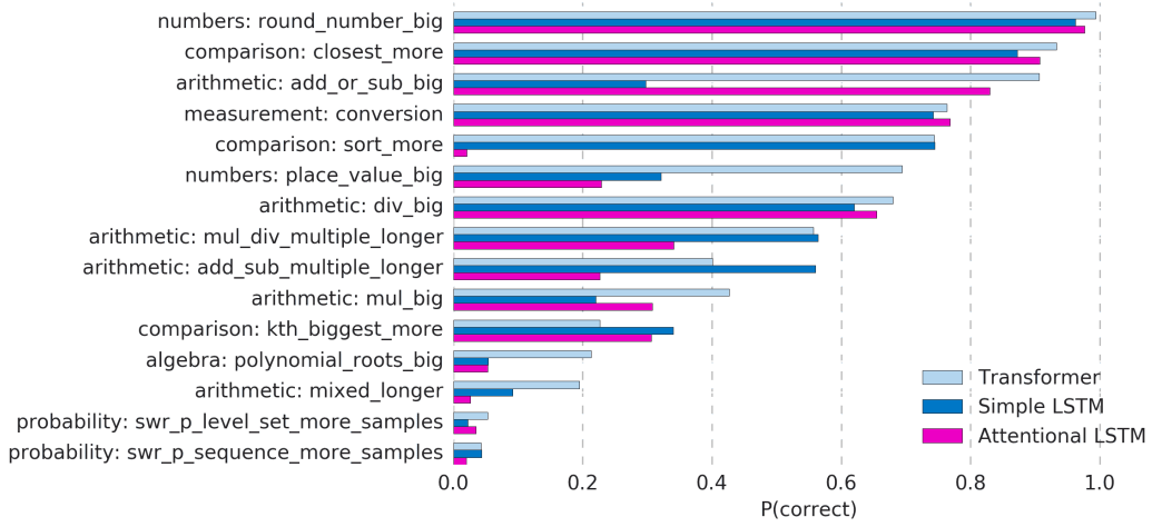
Figure 5: Extrapolation test performance on the different modules.
