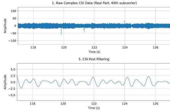
Fig. 2. CSI data before and after filtering
