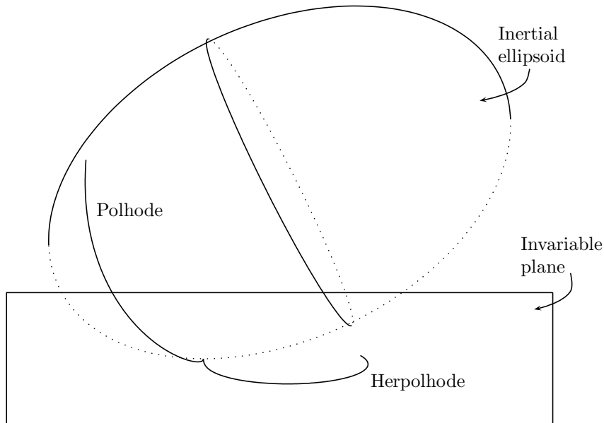
Figure 1: This figure shows the inertial ellipsoid, the invariable plane, the polhode and the herpolhode. The angular momentum is downward, so the invariable plane is horizontal. The herpolhode is a curve traced out on the invariable plane, and the polhode is a curve on the surface of the inertial ellipsoid.
