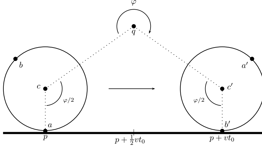
Figure 2: This shows the starting and stopping position of a disk which has rolled along the line. The rolling motion is equivalent to rotation by angle \varphi around the point q . The points a, b are fixed points on the circumference of the disk; the point c is the center of the disk. The positions of the points after the disk has finished rolling are labelled a', b', c' .
