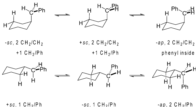
Scheme 12. Repulsive Gauche Interactions Present in the Axial and Equatorial Conformers of Benzylcyclohexane a
