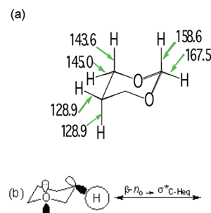
Figure 7. (a) Experimentally obtained one-bond coupling constants in 1,3-dioxane. 26 (b) Through-space hyperconjugative interaction between a p -type lone pair at the \beta -oxygen and the back lobe of the antibonding C(5)–H eq orbital. 29
