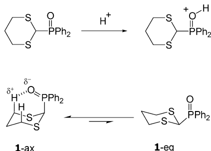
Scheme 5. Protonation of the Phosphoryl Oxygen under Strongly Acidic Conditions (Top) Is Likely To Turn off Some Electrostatic, Attractive Interaction in 1-ax (Bottom) 12c
