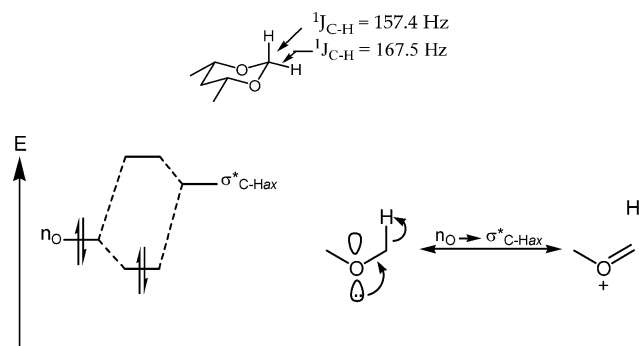
Scheme 7. Stereoelectronic Interpretation of the Smaller ^1J_{C-H} in the Axial C–H Bond Adjacent to Oxygen
