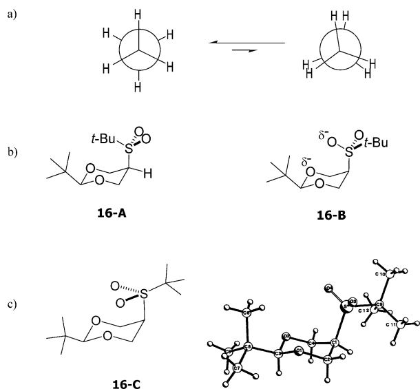
Scheme 11. (a) Preferred Staggered Conformation in Ethane. (b) Anticipated Staggered Rotamers in cis -16. (c) Solid-State Structure and Conformation of Heterocycle cis -16 33
