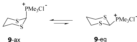
Scheme 6. A Definite Preference for the Axial Conformation 9-ax, \Delta G^\circ = +0.36 kcal/mol, Reflects a Substantial S–C– + PMe 3 Anomeric Effect in This System, Worth at Least 2.2 kcal/mol 19
