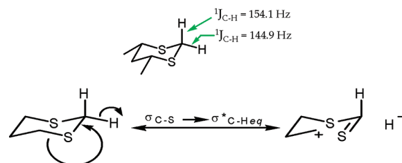
Scheme 8. Stereoelectronic Interpretation of the Smaller ^1J_{C-H} in the Equatorial C–H Bond Adjacent to Sulfur
