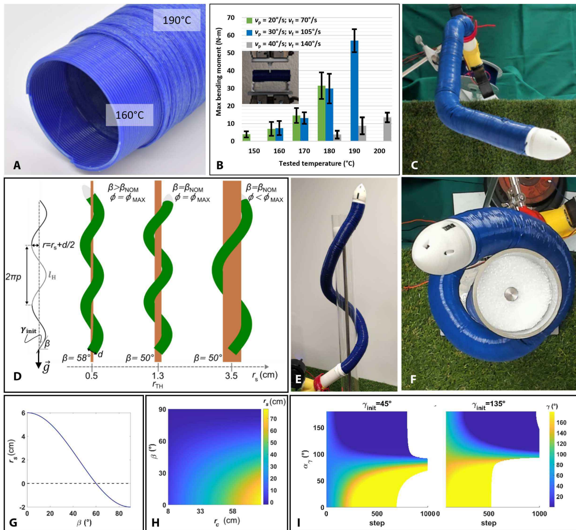
Fig. 3. Climbing plant-inspired behaviors in FiloBot. (A) A sample of a built structure where there is a passage between different printing parameters: from v_p = 30^\circ/s , v_f = 105^\circ/s , at 160^\circ\text{C} to v_p = 30^\circ/s , v_f = 105^\circ/s , at 190^\circ\text{C} . The higher temperature produced thinner layers with a larger width, showing stronger bonding. (B) Maximal bending moments achieved via three-point bending tests (inset) on stem-like structures generated using different plotting parameters. (C) Growth across a void. The final displacement in this experiment was 50 cm. (D) Three helical growth patterns simulated with different support radii and initial tip inclinations. The helical growth parameters are shown on the left. (E) Growth via twining with a support of 7-cm diameter and a helix slope angle of \beta = 50^\circ . (F) Aerial view of the robot in a twining configuration. (G) Maximal support radius as a function of \beta considering r_c = 8 cm. (H) Evaluation of maximal support radius varying helix inclination and curvature radius. (I) Variation of tip inclination ( \gamma ), given as examples two different initial inclinations ( \gamma_{\text{init}} ), when an offset ( \alpha_\gamma ) is applied to the growth direction \theta = \alpha_\beta + \alpha_\gamma . \alpha_\beta defines the direction to follow gravity.
