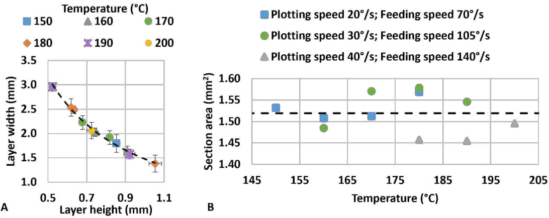
Fig. S 1. Results of different printing parameters. (A) Relation between layer height and width. In constant printing parameters (but variable values of temperature, feeding, and plotting speed), the body structure will be formed by almost constant layers and width ( w ) relates to height ( h ) with the law w = 1.48h^{-1.1} . (B) Obtained layer section area (dot data) and estimated average (dashed line) over different plotting and feeding speeds and temperatures.
