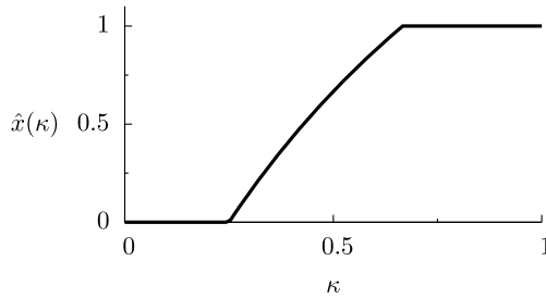
FIGURE 1.—The (singleton) set of homo moralis strategies for (T, R, P, S) = (7, 5, 3, 2) .
