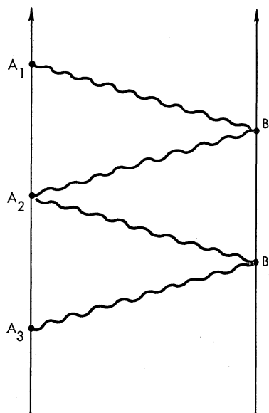
FIG. 4. A and B use tachyonic antitelephones to communicate backwards in time. A message sent by A at 3:00 o'clock ( A_1 ) is received by B at 2:00 o'clock ( B_1 ), etc.
