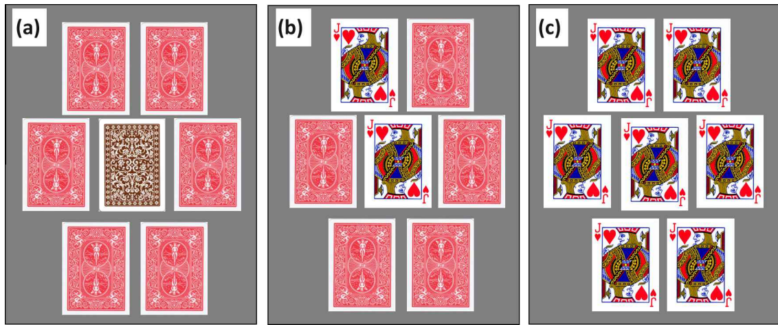
Fig. 1. Configuration of the seven face down cards (a). A chosen card and the matching prediction (b). Secret of the trick (c).
