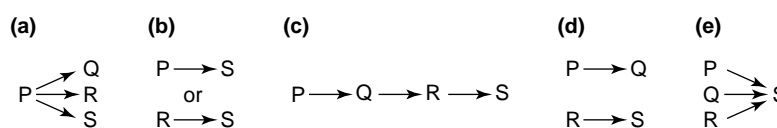
Fig. 1. The causal-status effect predicts biases to favour some causal patterns over others as diagnostic of important causal features, most notably the initiating causal factor in a chain. That effect might in turn spring from an essentialist bias for natural kinds in which a single common cause is thought to produce effects. Adults and children alike seem to expect that natural kinds will be explainable by a set of structured relations of the form shown in (a), as opposed to the other possibilities shown in (b–e) [53]. Whereas property P in case (c) would also be predicted to be more central than Q, R or S by causal status, property P in case (a) is especially salient as the initiator of three distinct effects. Adapted with permission from [53].
