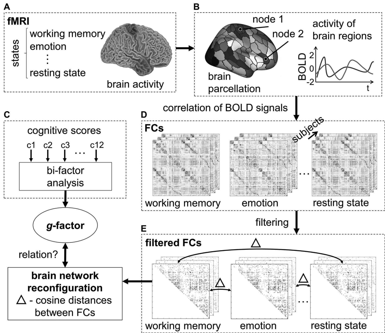
Figure 1. Schematic overview of global analysis workflow. (A) Brain activity was assessed with fMRI during eight different cognitive states (resting state and seven tasks). (B) For each state, functional brain connectivity matrices (FCs, D) were computed by correlating the time series of 200 nodes with each other. For noise reduction, FCs were filtered based on their correlation with intelligence (see Supplementary Fig. 1 and Materials and Methods for details). Brain network reconfiguration was calculated for all state combinations as cosine distances ( \Delta ) between the filtered FCs (E). To assess the relationship between brain network reconfiguration and intelligence, reconfiguration values were correlated (Spearman correlations, controlled for age, sex, handedness, and in-scanner head motion) with a latent g -factor derived from 12 cognitive scores using a bi-factor analysis model (C). t, time; c, cognitive score.
