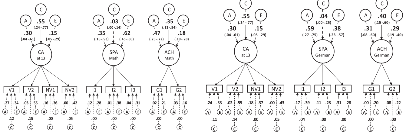
Fig. 1. Results of common-pathway model analyses of genetic (A), shared environmental (C), and nonshared environmental (E) influences on the latent factors of CA, SPAs, and ACH for Math (a) and German (b). The path estimates of common A, C, and E influences on CA, SPA and ACH are shown in the upper section of each diagram. Numbers in parentheses reflect 95% confidence intervals. Path estimates of specific A, C, and E influences are shown in the bottom section of each diagram (95% confidence intervals are given in Fig. 2). All path estimates are standardized and squared to refer to the percentage of variance explained, non-significant paths are represented as dashed lines.
