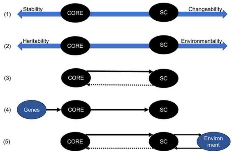
Fig. 1. (Color online) Illustration of the five criteria to conceptually and empirically differentiate between core personality (CORE) and surface characteristics (SC): Core characteristics are (1) more stable, (2) less environmentally malleable, (3) they shape surface characteristics rather than vice versa, (4) genetic variance in surface characteristics should be completely accounted for by genetic variance in core characteristics and (5) surface characteristics mediate the effects from core characteristics on the environment (selection effects) and vice versa (socialization effects).
