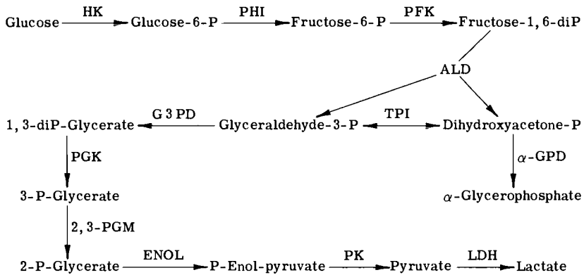
FIG. 2. Enzymatic steps of the glycolytic pathway: hexokinase (HK), phosphohexose isomerase (PHI), phosphofruktokinase (PFK), aldolase (ALD), triosephosphate isomerase (TPI), glyceraldehyde-3-phosphate dehydrogenase (G3PD), phospho-glycerate kinase (PGK), 2,3-phosphoglycerate mutase (2,3-PGM), enolase (ENOL), pyruvate kinase (PK), and lactate dehydrogenase (LDH). In addition, \alpha -glycerophosphate dehydrogenase ( \alpha GPD) is shown.
