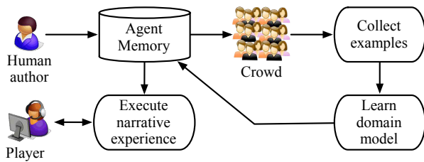
Figure 1: The SCHEHERAZADE-IF architecture.
