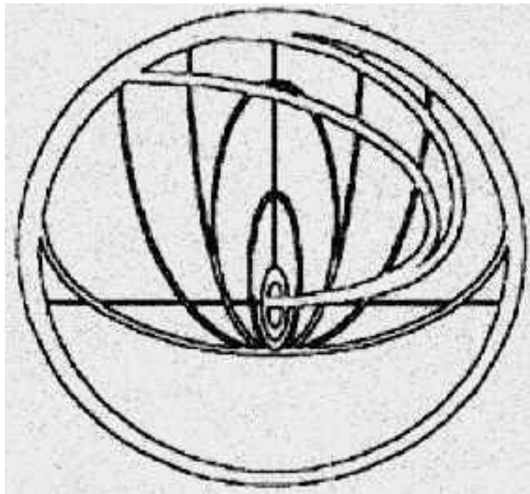
Figure 1.2: The alleged insignia of John Titor's time travel group. The ring singularity of a Kerr black hole is represented, with two paths through indicated: a safe route and a "path to God".
