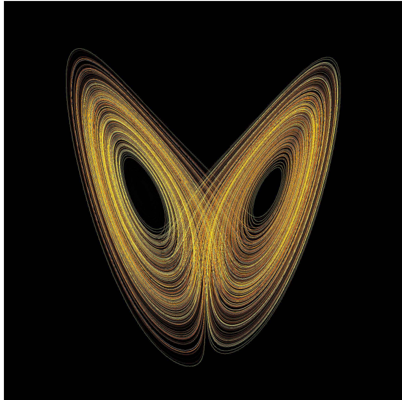
Figure 1.1: The strange attractor of the Lorenz system . Lines illustrate the paths that systems take through parameter space, as they evolve with time. Despite the chaotic dynamics, they continue to orbit the attractor. (By Wikimol on Wikimedia .)
