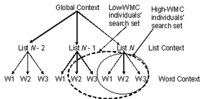
Figure 2. Depiction of high and low WMC individuals' search sets on the basis of contextual cues used at retrieval. Individuals rely on the current contextual state to retrieve items from the current list (List N ). However, noisy list context cues tend to activate items from the immediately preceding list (List N - 1 ), leading to the inclusion of interfering item representations from previous trials in the search set. WMC = working memory capacity; W = word.
