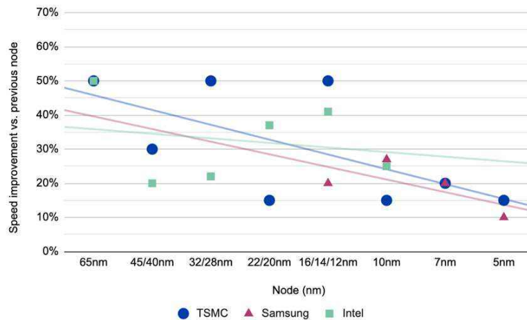
Figure 5: Node-to-node transistor speed improvements
