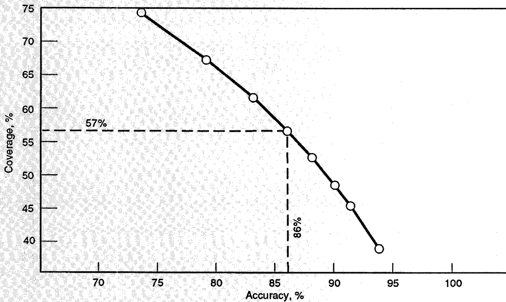
Figure 2. Threshold calculations for coverage and accuracy
