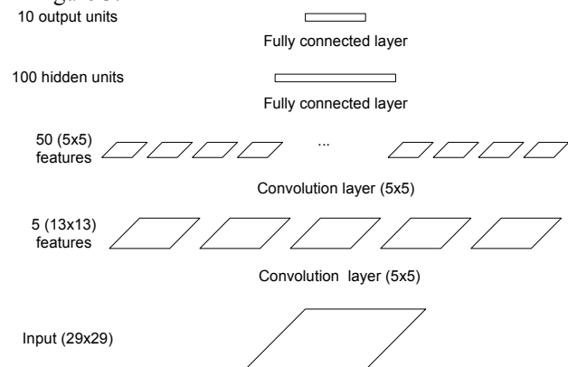
Figure 3. Convolution architecture for handwriting recognition
