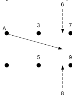
Figure 1. How to compute new grey level for A, at location (0,0) given a displacement \Delta x(0,0) = 1.75 and \Delta y(0,0) = -0.5 . Bilinear interpolation yields 7.0.
